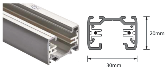
Single circuit track (/1CT)
