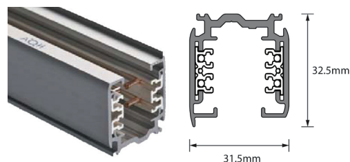
Three circuit track (/3CT)
