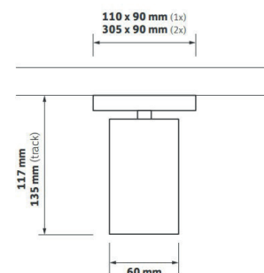
Side View Profile Dimensions
