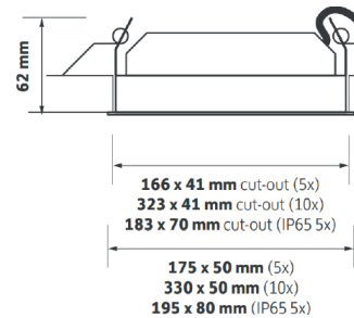
Side Profile View Dimensions
