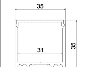
LEX/S/B dimensions
