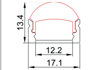
LEX/S/60D dimensions
