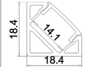
LEX/MID007-R dimensions
