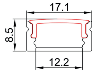
LEX/S dimensions
