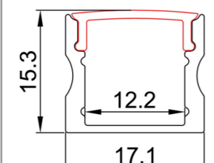
LEX/MID004-R dimensions
