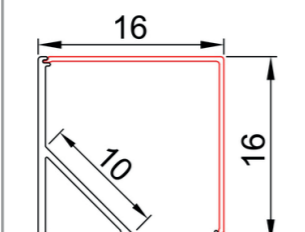
LEX/S/B45D dimensions
