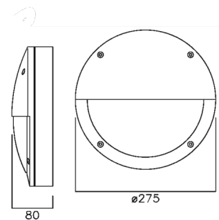
Front and Side View Dimensions
