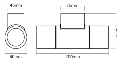
Side View Dimensions
