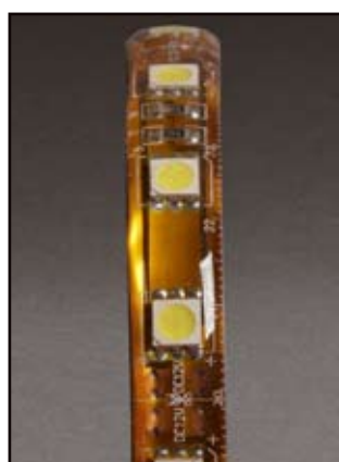
IP67 rated 60 LEDs/m - 4.8W/m
